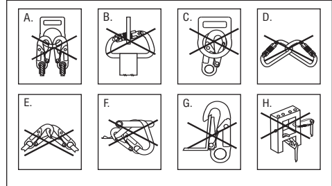
Fig. 3 - Inappropriate Connections
