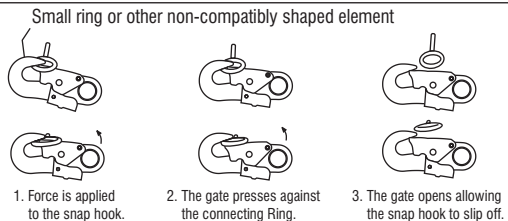
Fig. 3 - Inappropriate Connections
